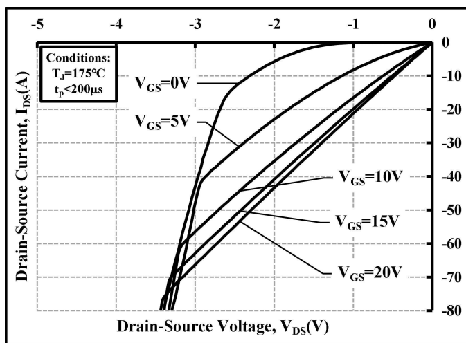
Figure 12: 3rd Quadrant Characteristic at 175°C
