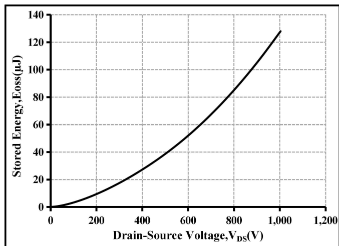
Figure 13: Output Capacitor Stored Energy
