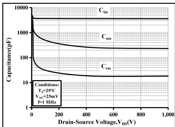
Figure 15: Capacitance vs Drain-Source Voltage (0-1000 V)
