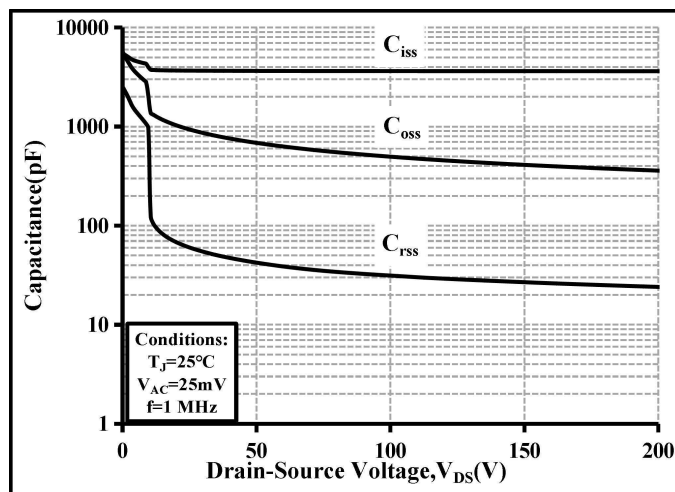
Figure 14: Capacitance vs Drain-Source Voltage (0-200 V)
