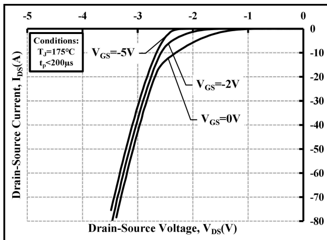
Figure 8: Body Diode Characteristic at 175°C
