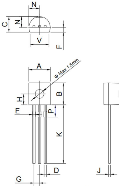
TO-92
