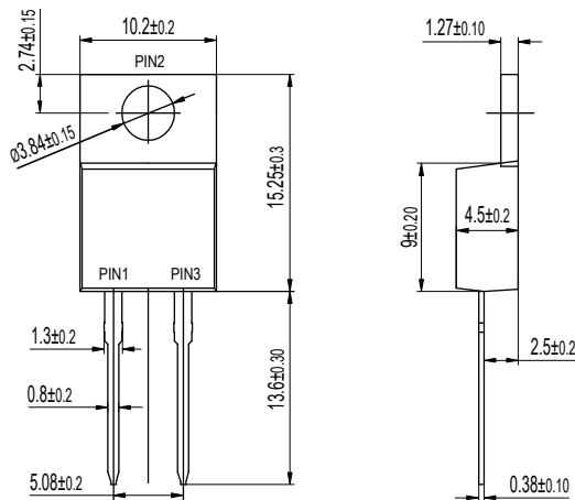
TO-220AC MBR20XX
