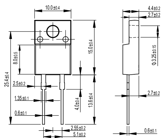
ITO-220AC MBR20XXF
