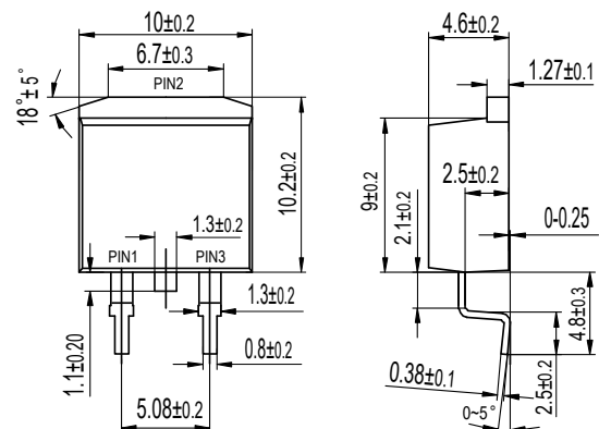
TO-263(D 2 PAK) MBR20XXD/D1
