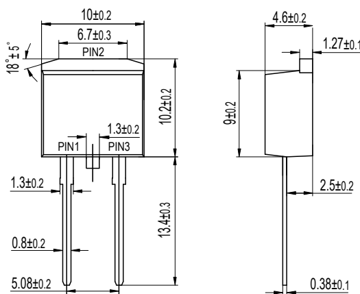
TO-262AC MBR20XXW
