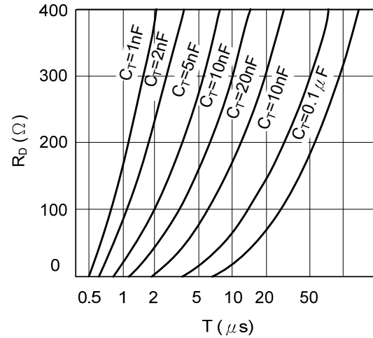
Oscillator DisCharge Time vs. R_D and C_T
