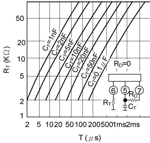
Oscillator Charge Time vs. R_T and C_T
