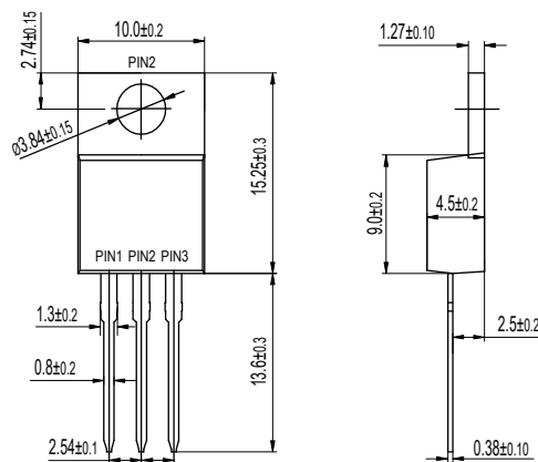
TO-220AB MBR30XXCT
