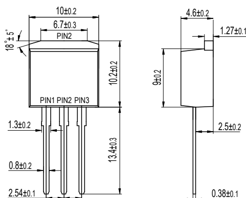
TO-262AB MBR30XXWCT
