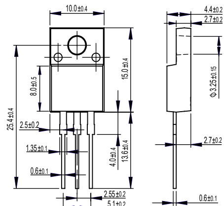
ITO-220AB MBR30XXFCT
